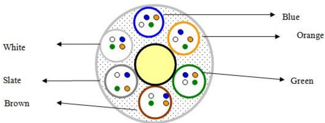
Color coding of Loose Tubes for 24 fibres (Refer Table - 1)
